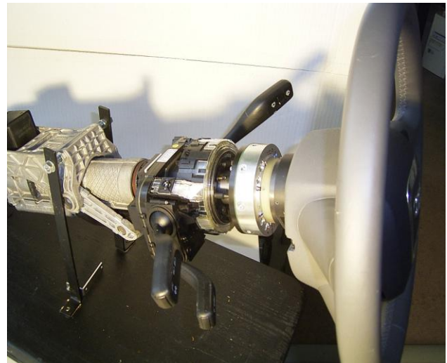
KMT-CLS Sensor in a standard application, located between steering wheel and steering column
